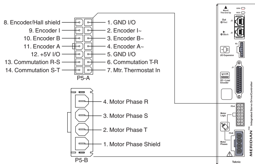
Motor Connectors P5-A and P5-B (M6xx/M7xx models)
