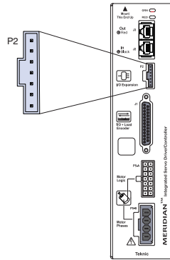
Meridian Expansion Connector (P2)
