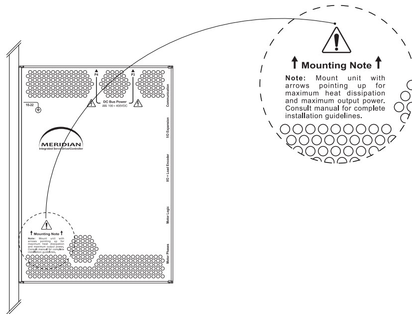
Meridian drive mounting orientation
