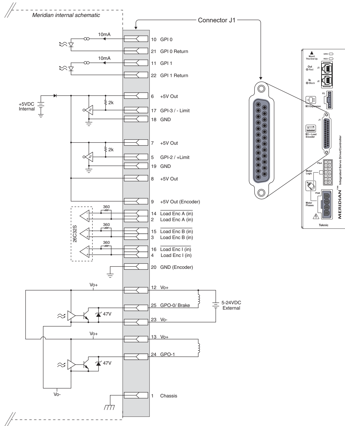
Meridian controller connector (J1) and schematic fragments
