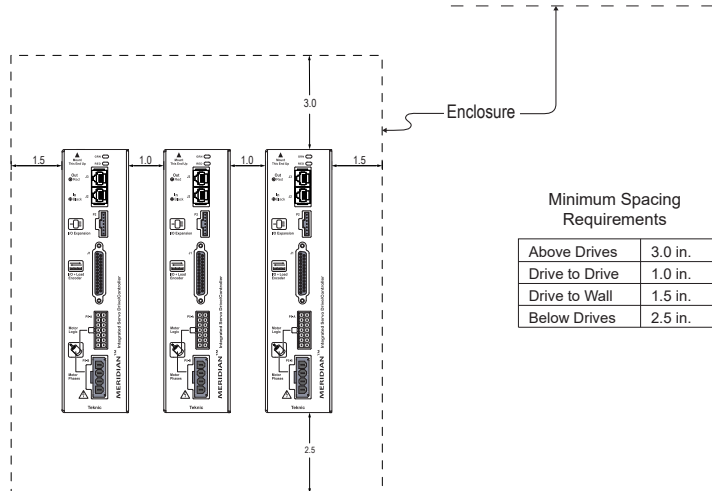
Mounting and clearance dimensions (M6xx/M7xx models)
