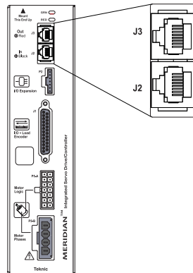
Meridian Diagnostic and Application Communications Connectors
