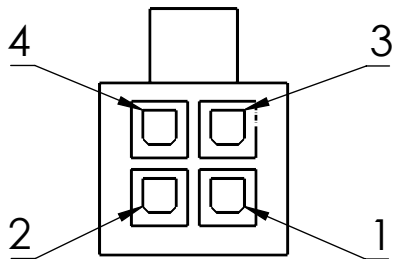
P1 Molex Micro-Fit 3.0 4-Position Wire Entry View Scale 3:1
