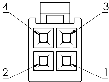
P1 Molex Mini-Fit Jr. 4-Position Wire Entry View Scale 3:1
