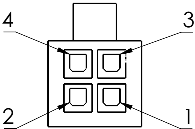
P2 Molex Micro-Fit 3.0 4-Position Wire Entry View Scale 3:1
