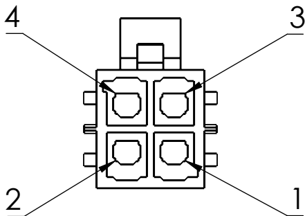
P1 Molex Micro-Fit+ Versa Color (Blue) 4-Position
