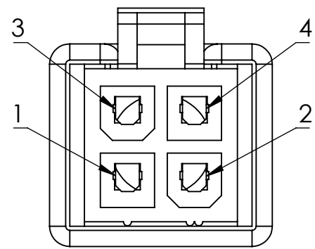
P1 Molex Mini-Fit Jr. 4
