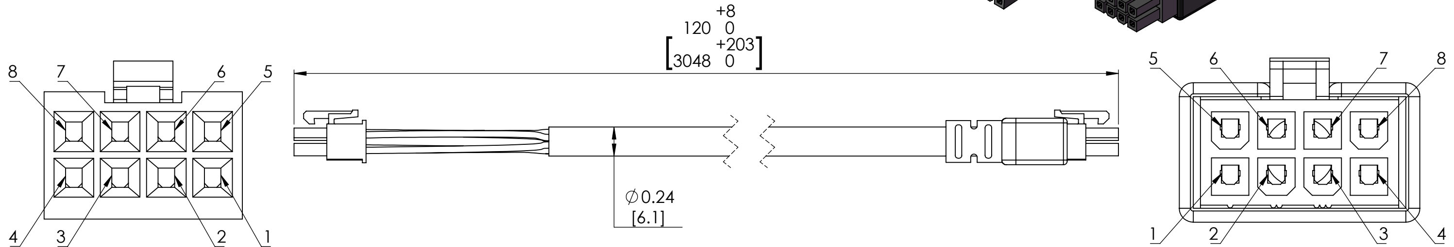
P1 Molex Mini-Fit Jr. 8 Wire Entry View Scale 3:1
